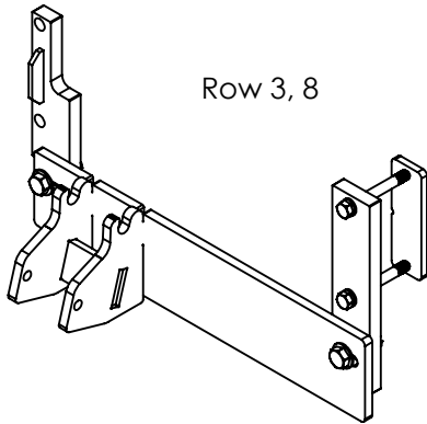
GRH7000-P
