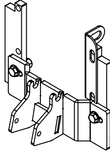
GRH7000-L
