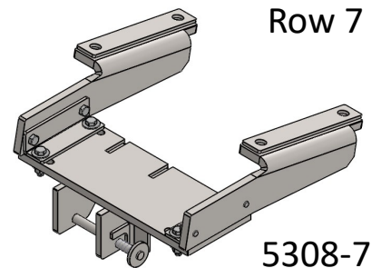
Row 7 mount installation
