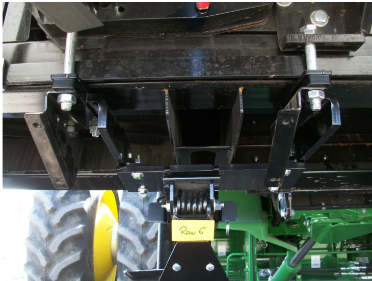
Rows 6 and 8 mount installation
