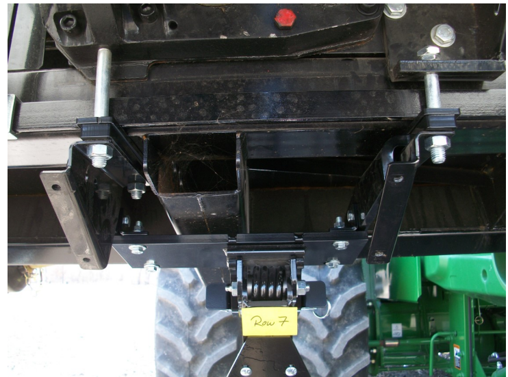
Row 7 mount installation
