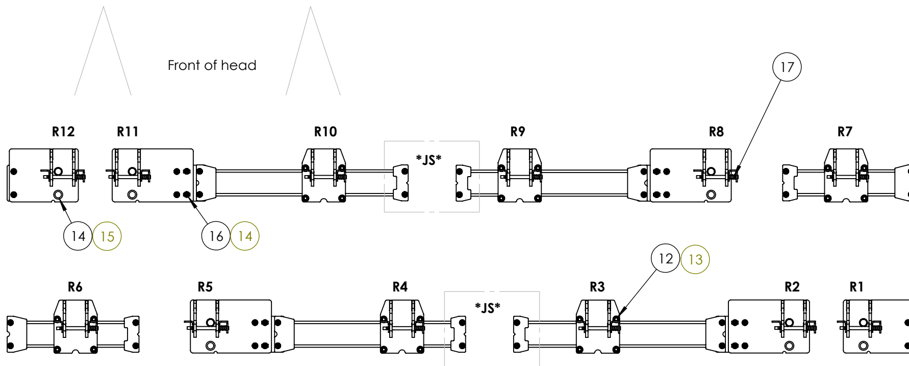
Bottom View
