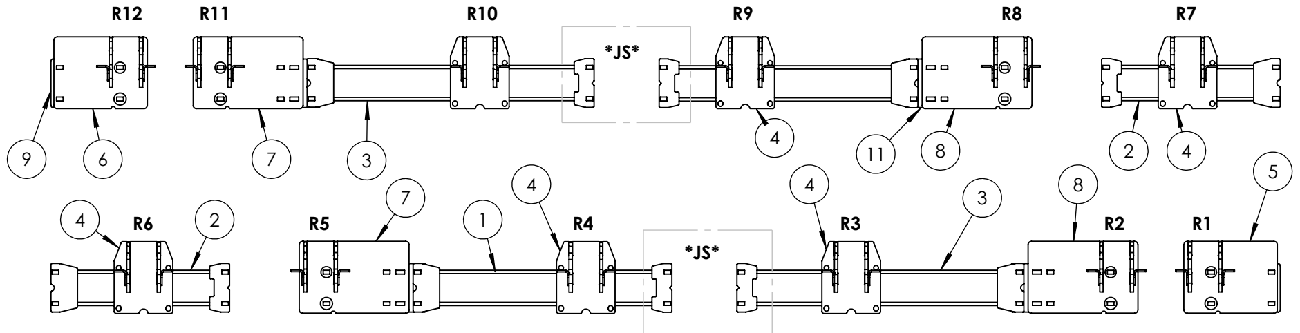
Bottom View
